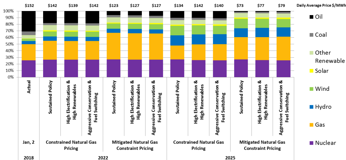
Figure 14: Severe Cold Day Fuel Mix Comparison
