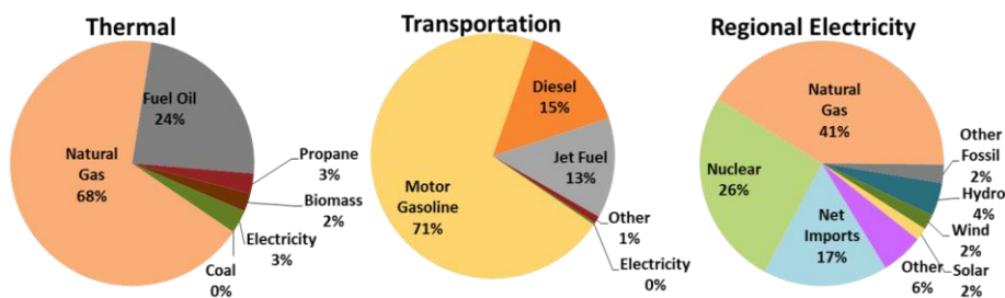
Figure 1: Massachusetts Energy Demand and Fuel Mix by Sector - 2016 5
