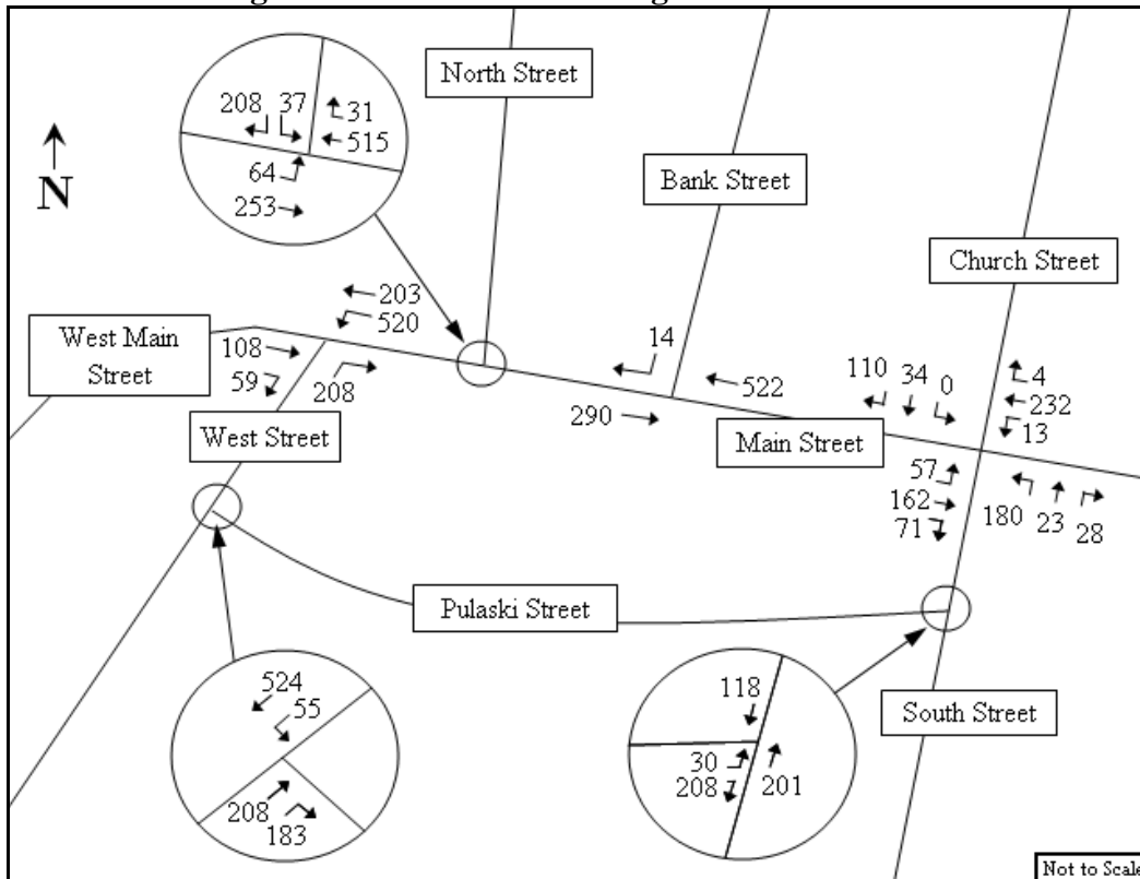
Figure II-2-PM Peak Turning Movement Count
